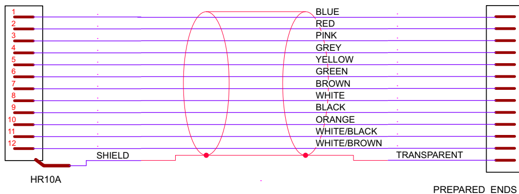
Figure 2: Guppy PRO cable color-coding
